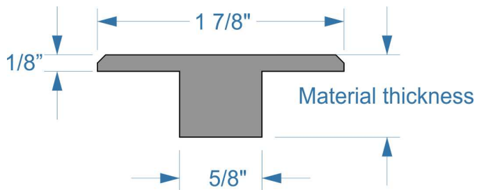
LTM1 - T-mould 1, wide
