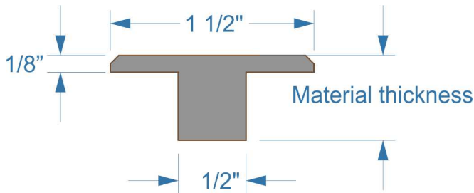
LTM2 - T-mould 2, narrow
