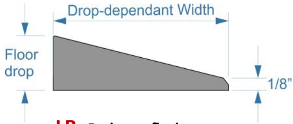
LR Reducer, flush
