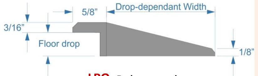
LRO Reducer, overlap
