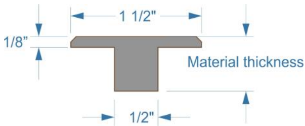
LTMS T-mould, small
